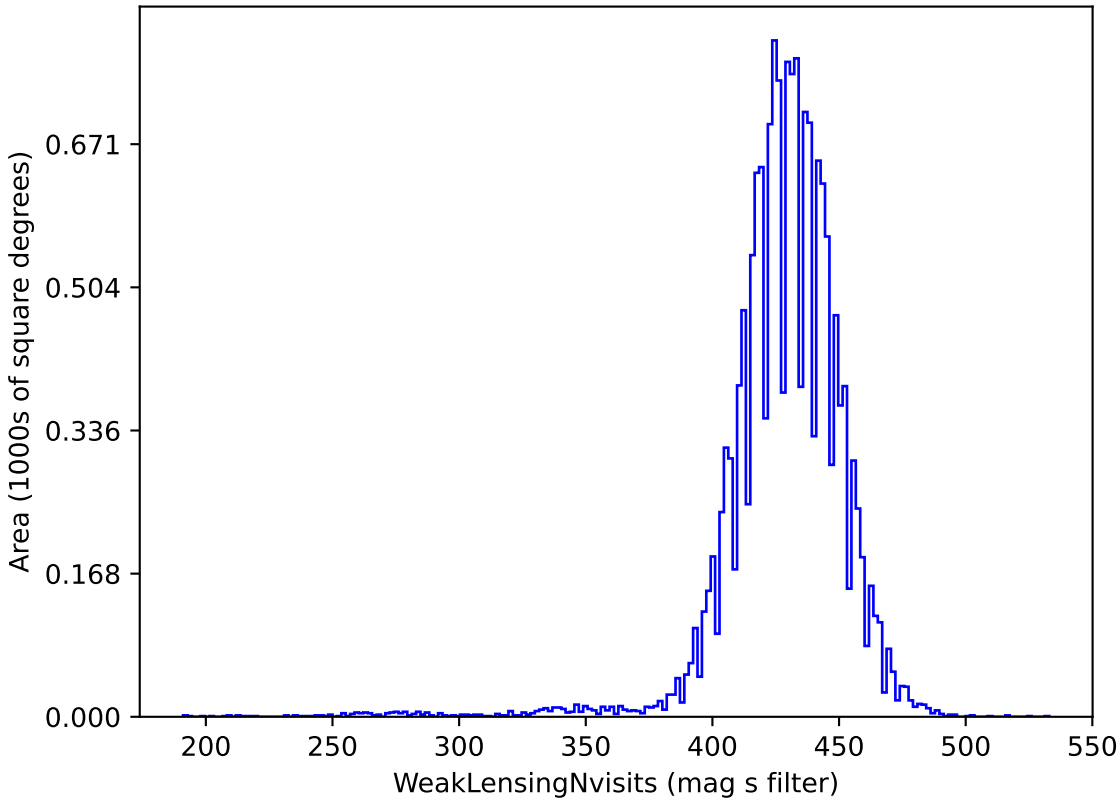
early_u_fpextra4.0_v3.4_10yrs gri band non-DD: WeakLensingNvisits
