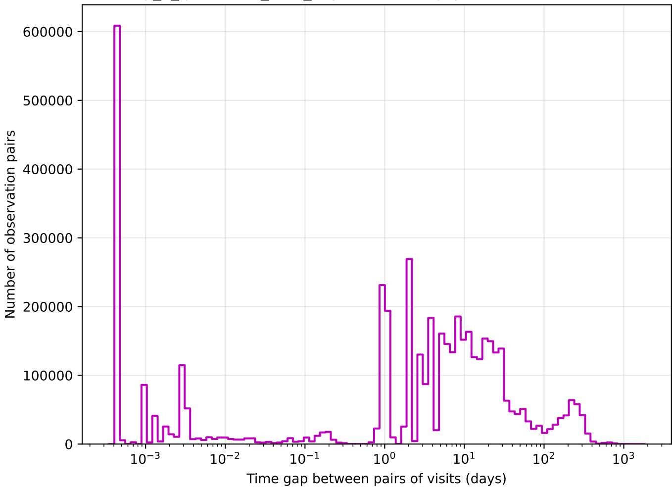
early_u_fpextra4.0_v3.4_10yrs z band: Tgaps observationStartMJD
