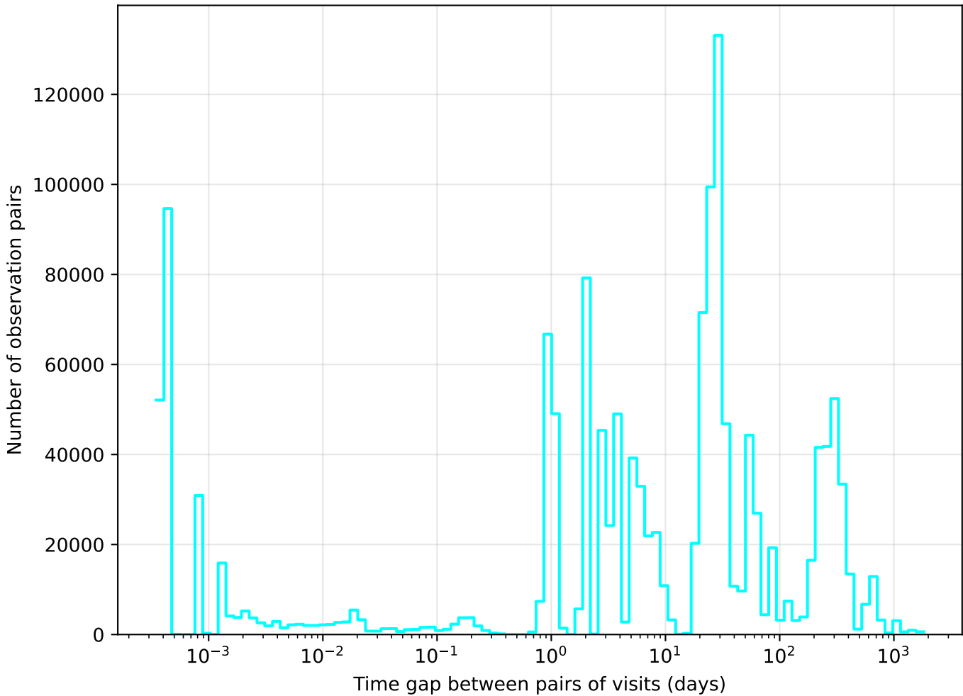
early_u_fpextra4.0_v3.4_10yrs u band: Tgaps observationStartMJD
