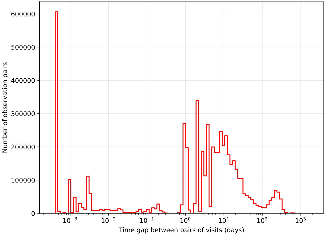
early_u_fpextra4.0_v3.4_10yrs i band: Tgaps observationStartMJD
