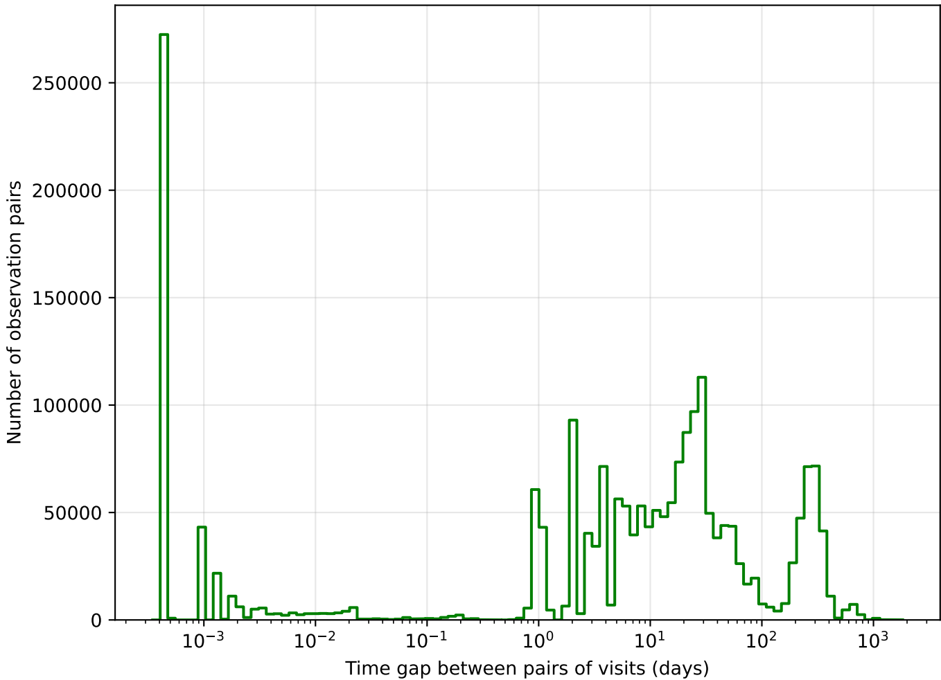
early_u_fpextra4.0_v3.4_10yrs g band: Tgaps observationStartMJD
