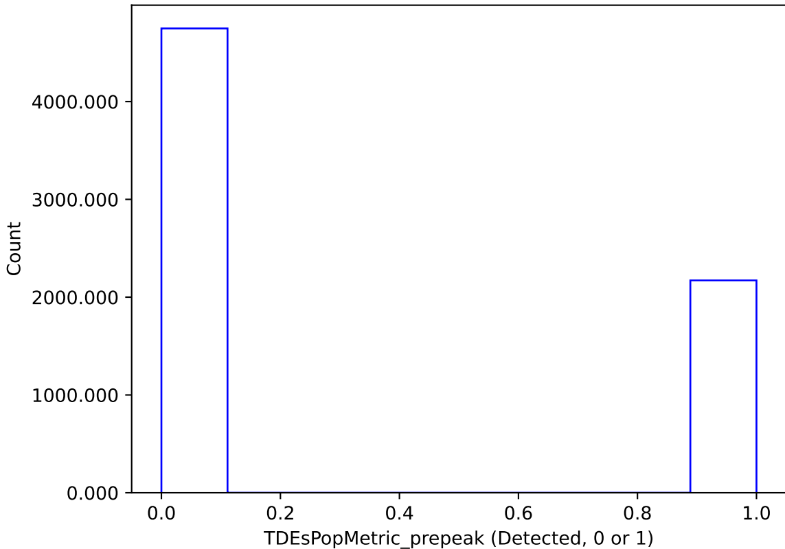
early_u_fpextra4.0_v3.4_10yrs : TDEsPopMetric_prepeak
