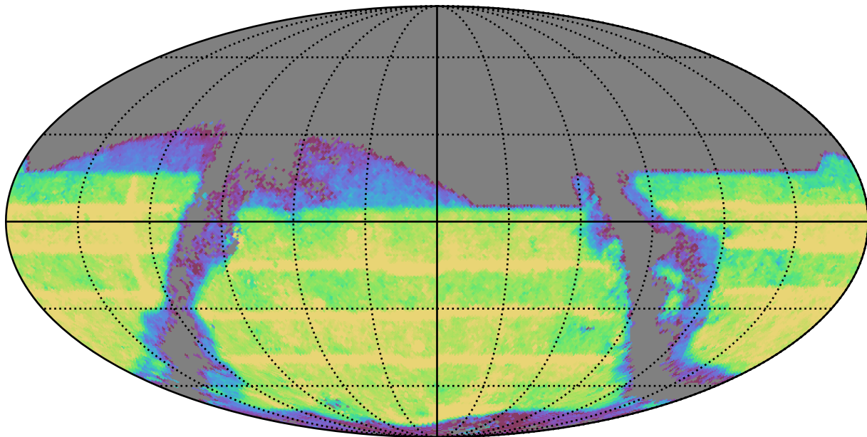
early_u_fpextra4.0_v3.4_10yrs : TDC_rate
