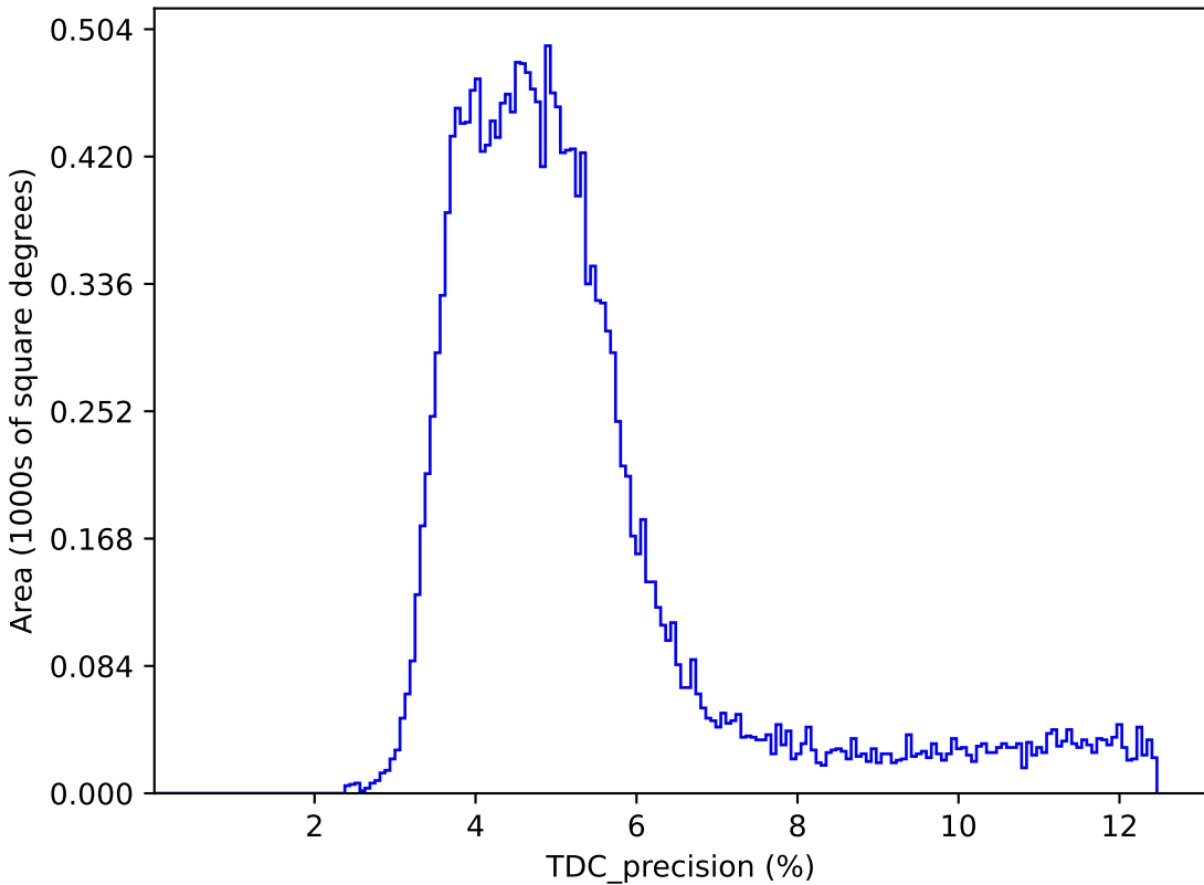
early_u_fpextra4.0_v3.4_10yrs : TDC_precision
