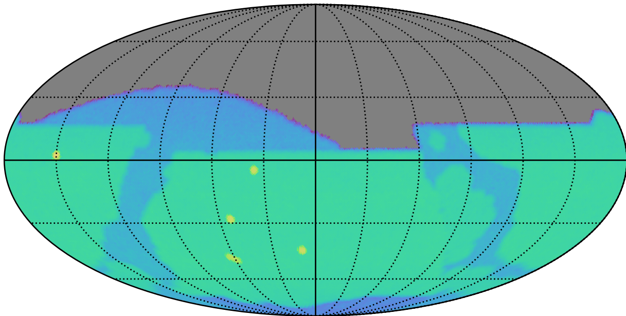
early_u_fpextra4.0_v3.4_10yrs z: SurfaceBrightLimit
