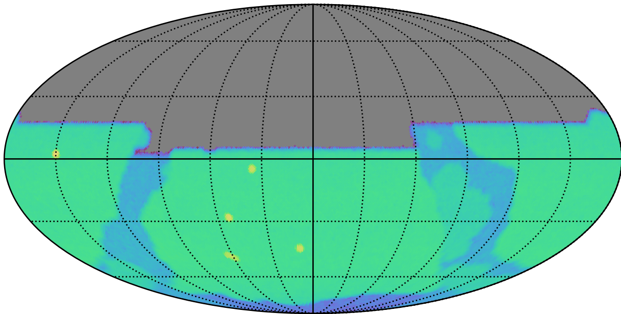
early_u_fpextra4.0_v3.4_10yrs y: SurfaceBrightLimit
