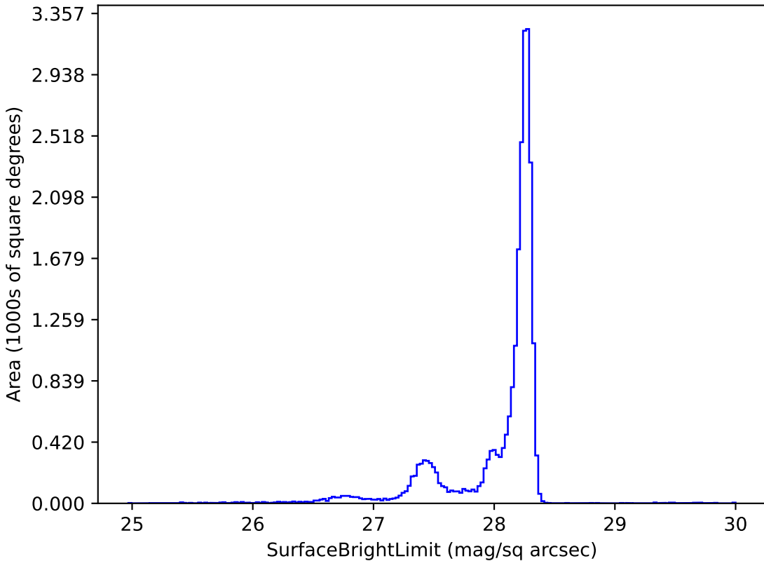
early_u_fpextra4.0_v3.4_10yrs y: SurfaceBrightLimit
