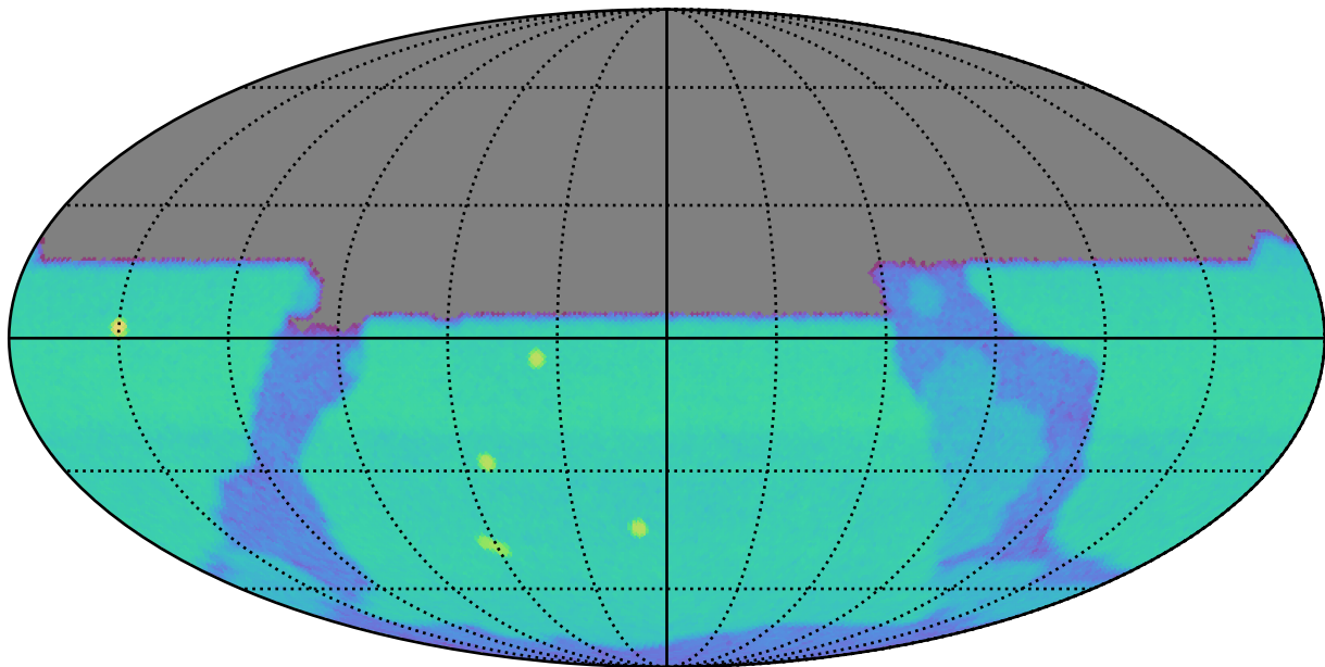
early_u_fpextra4.0_v3.4_10yrs u: SurfaceBrightLimit
