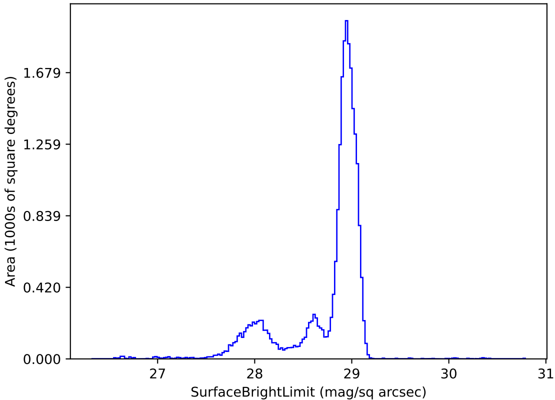
early_u_fpextra4.0_v3.4_10yrs u: SurfaceBrightLimit
