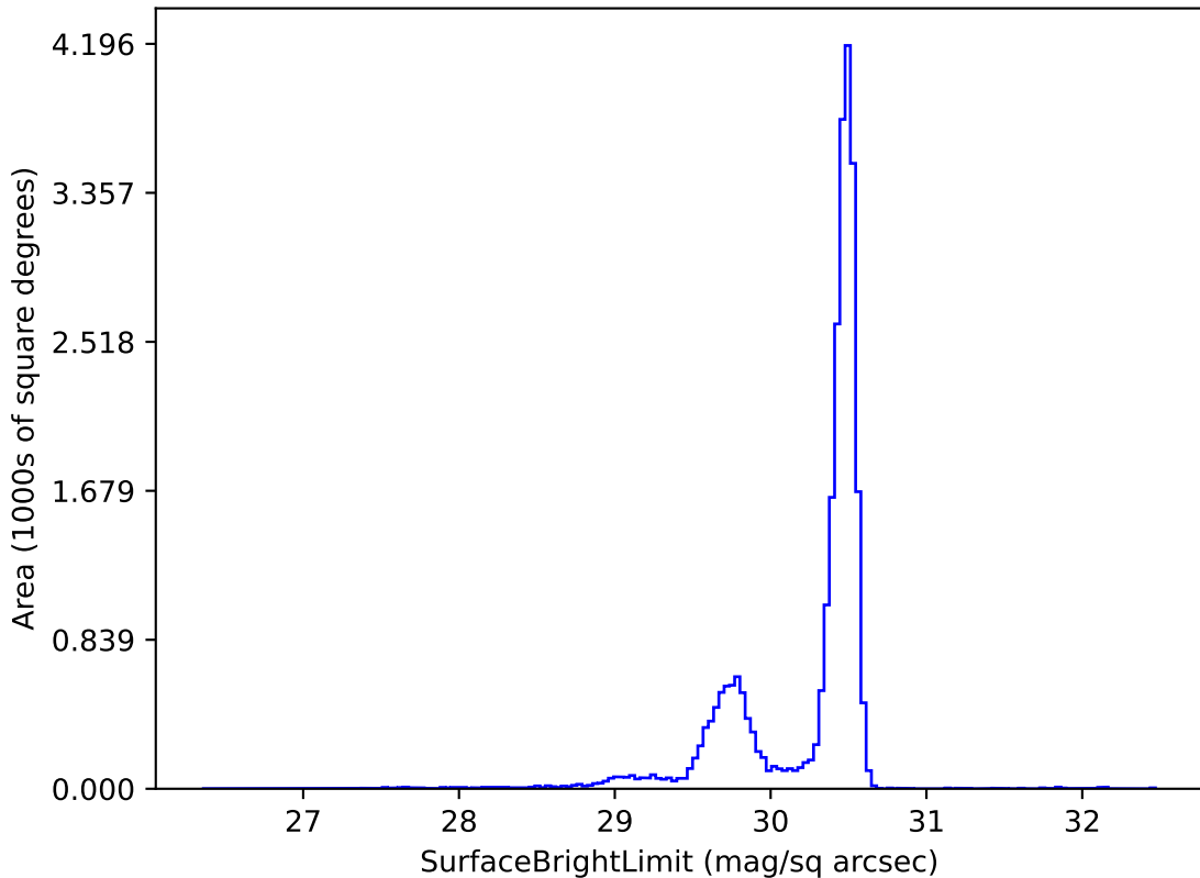
early_u_fpextra4.0_v3.4_10yrs r: SurfaceBrightLimit
