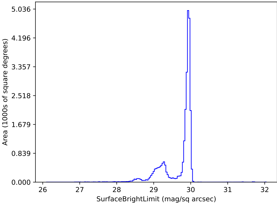
early_u_fpextra4.0_v3.4_10yrs i: SurfaceBrightLimit
