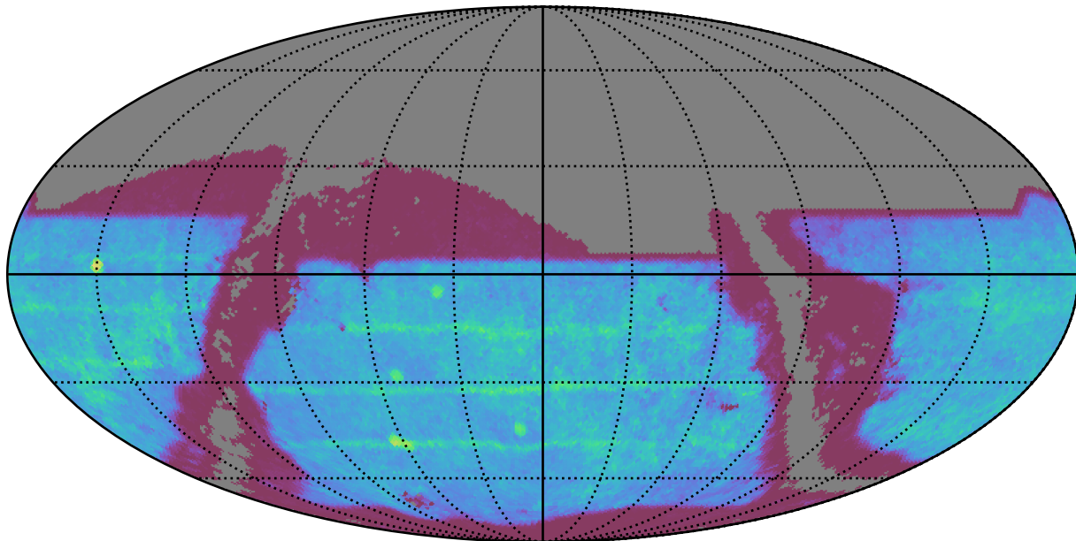
early_u_fpextra4.0_v3.4_10yrs : SNSLMetric
