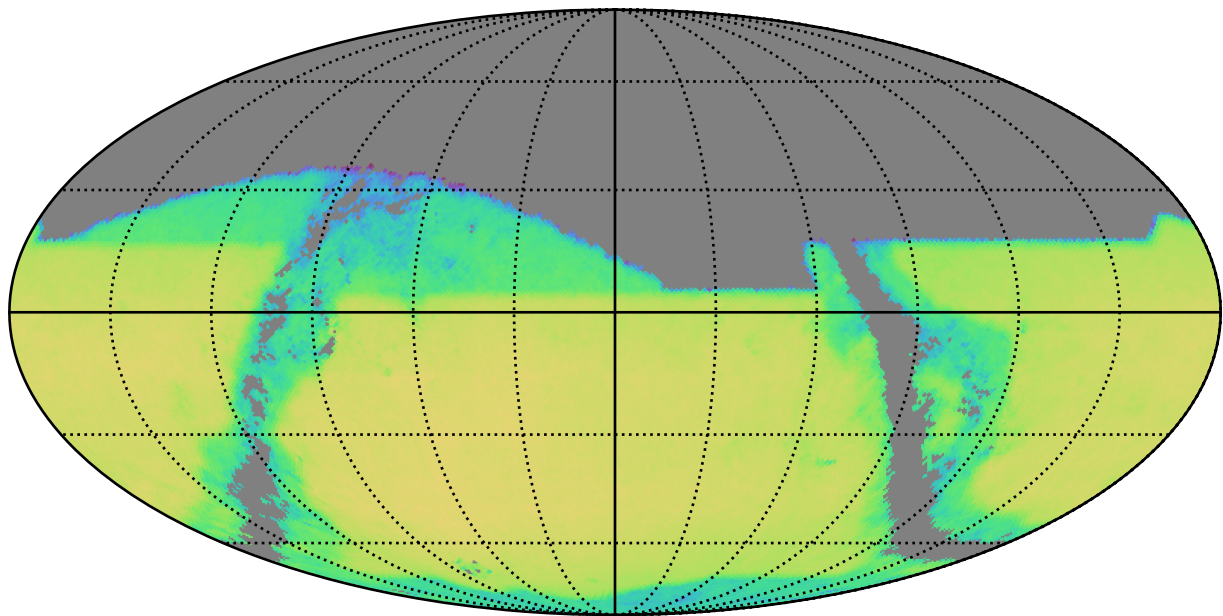
early_u_fpextra4.0_v3.4_10yrs z band and non-DD: QSONumberCountsMetric
