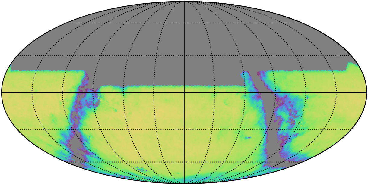
early_u_fpextra4.0_v3.4_10yrs u band and non-DD: QSONumberCountsMetric
