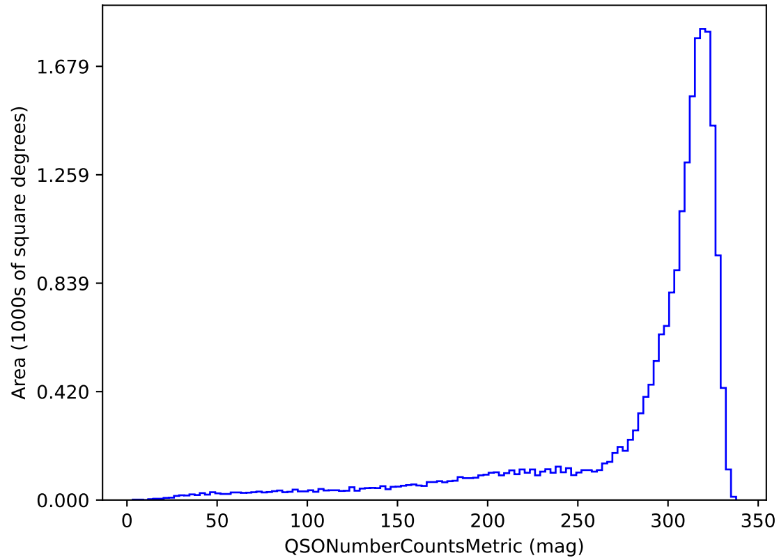
early_u_fpextra4.0_v3.4_10yrs u band and non-DD: QSONumberCountsMetric
