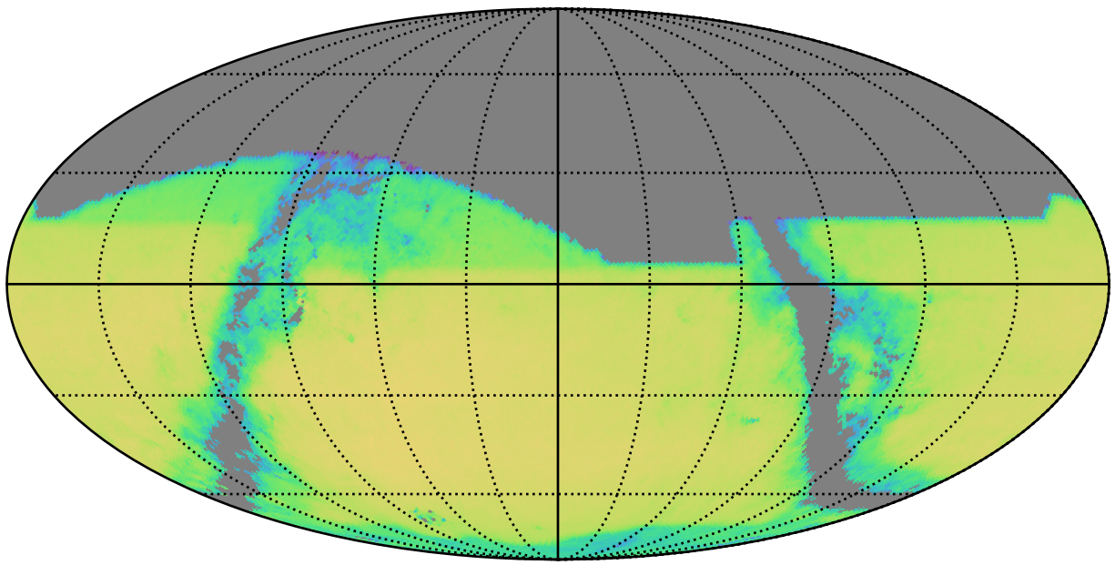
early_u_fpextra4.0_v3.4_10yrs r band and non-DD: QSONumberCountsMetric
