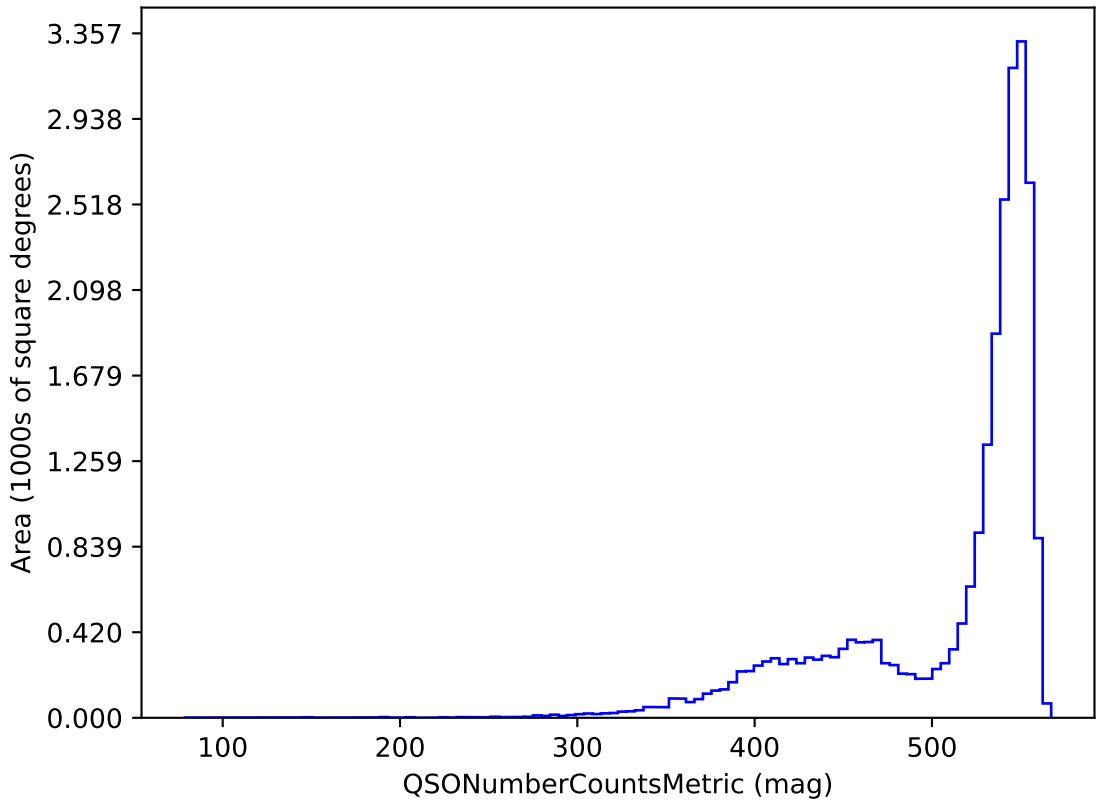
early_u_fpextra4.0_v3.4_10yrs i band and non-DD: QSONumberCountsMetric
