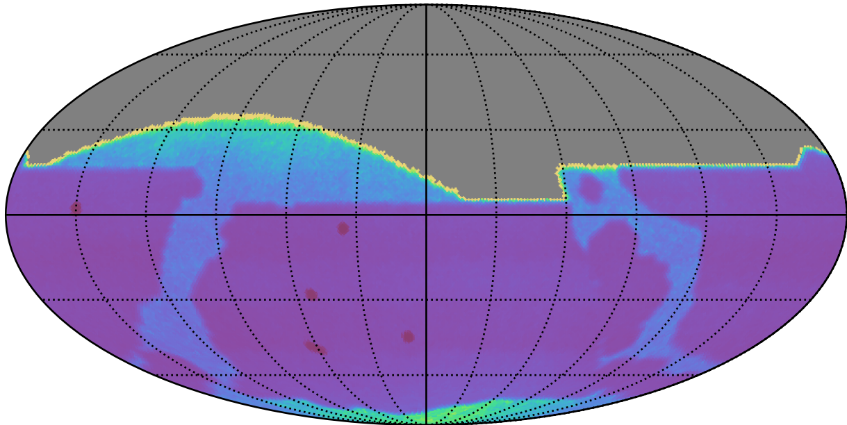
early_u_fpextra4.0_v3.4_10yrs : Proper Motion Uncert @ 20.5
