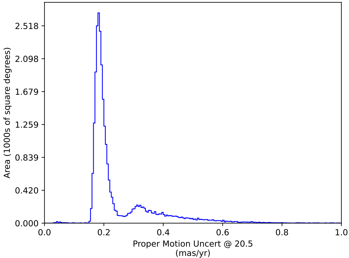
early_u_fpextra4.0_v3.4_10yrs : Proper Motion Uncert @ 20.5
