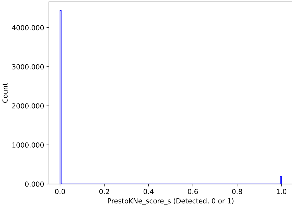
early_u_fpextra4.0_v3.4_10yrs : PrestoKNe_score_s
