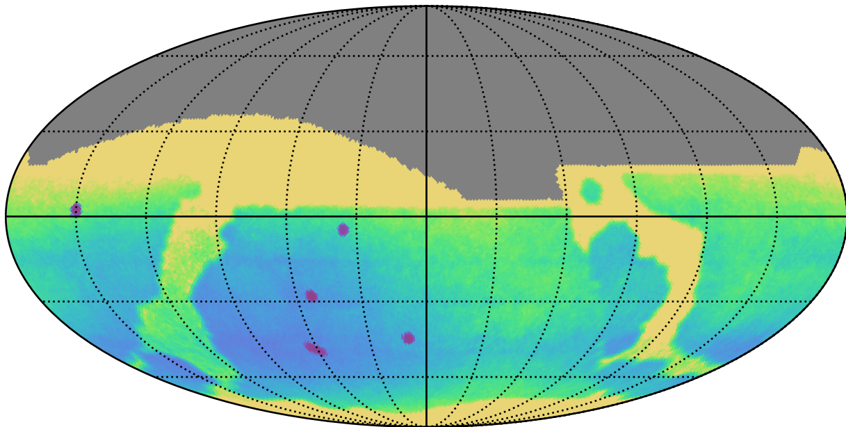
early_u_fpextra4.0_v3.4_10yrs : Parallax Uncert @ 24.0
