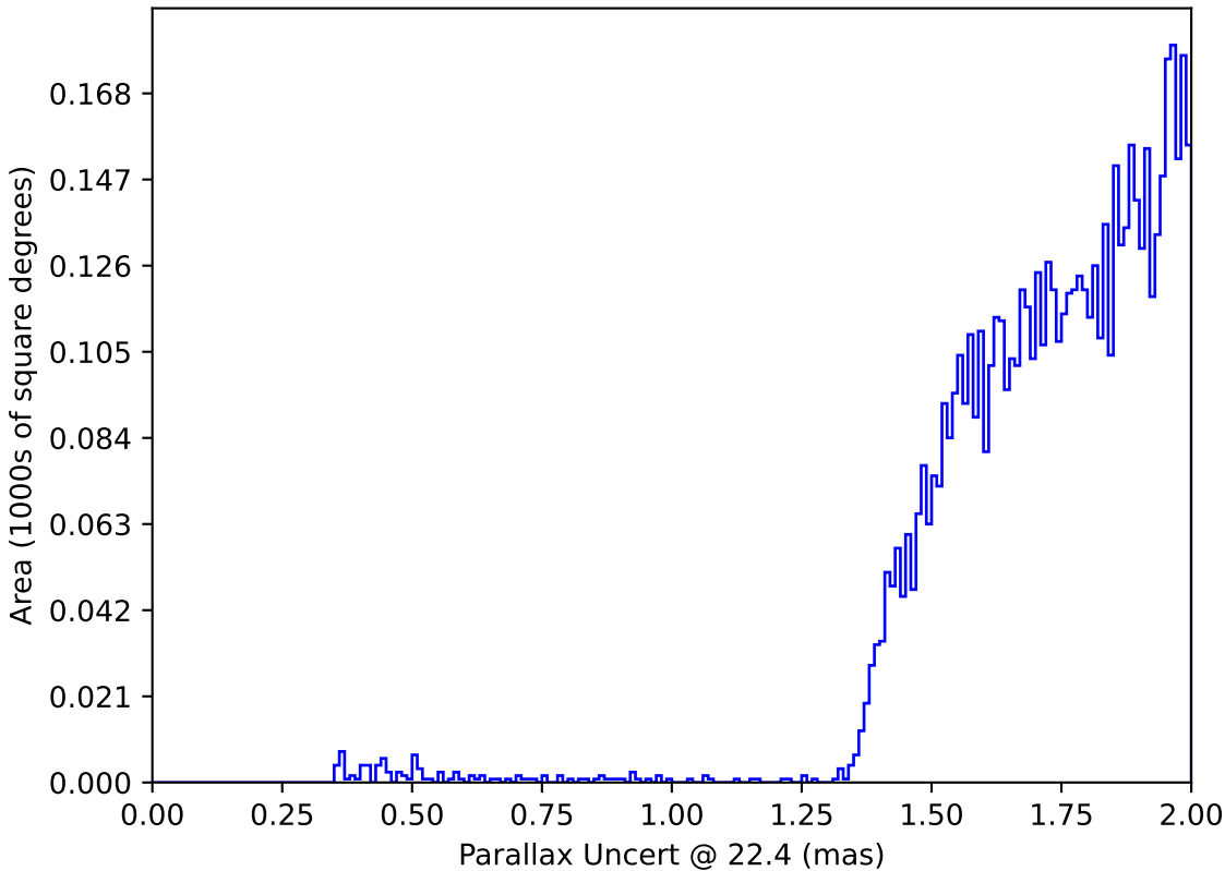
early_u_fpextra4.0_v3.4_10yrs : Parallax Uncert @ 22.4
