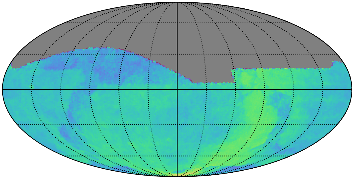
early_u_fpextra4.0_v3.4_10yrs : Parallax Coverage @ 24.0
