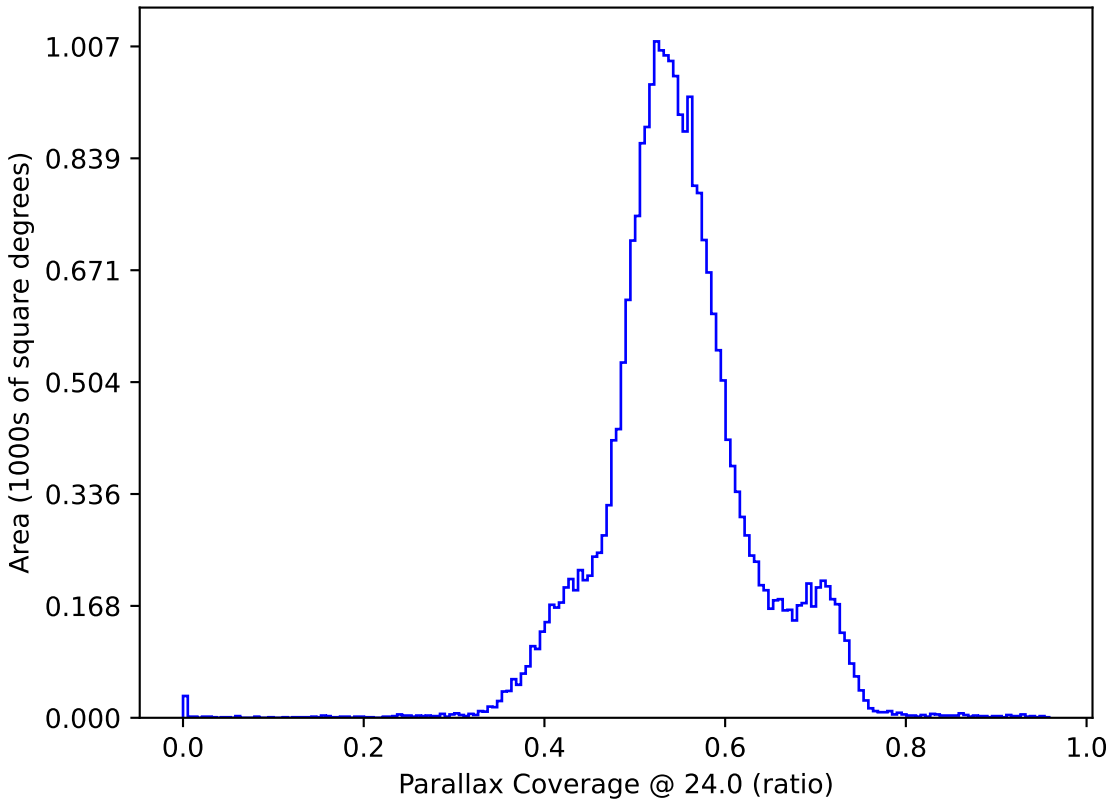
early_u_fpextra4.0_v3.4_10yrs : Parallax Coverage @ 24.0
