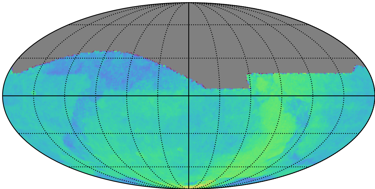
early_u_fpextra4.0_v3.4_10yrs : Parallax Coverage @ 22.4
