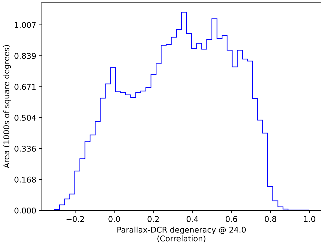
early_u_fpextra4.0_v3.4_10yrs : Parallax-DCR degeneracy @ 24.0
