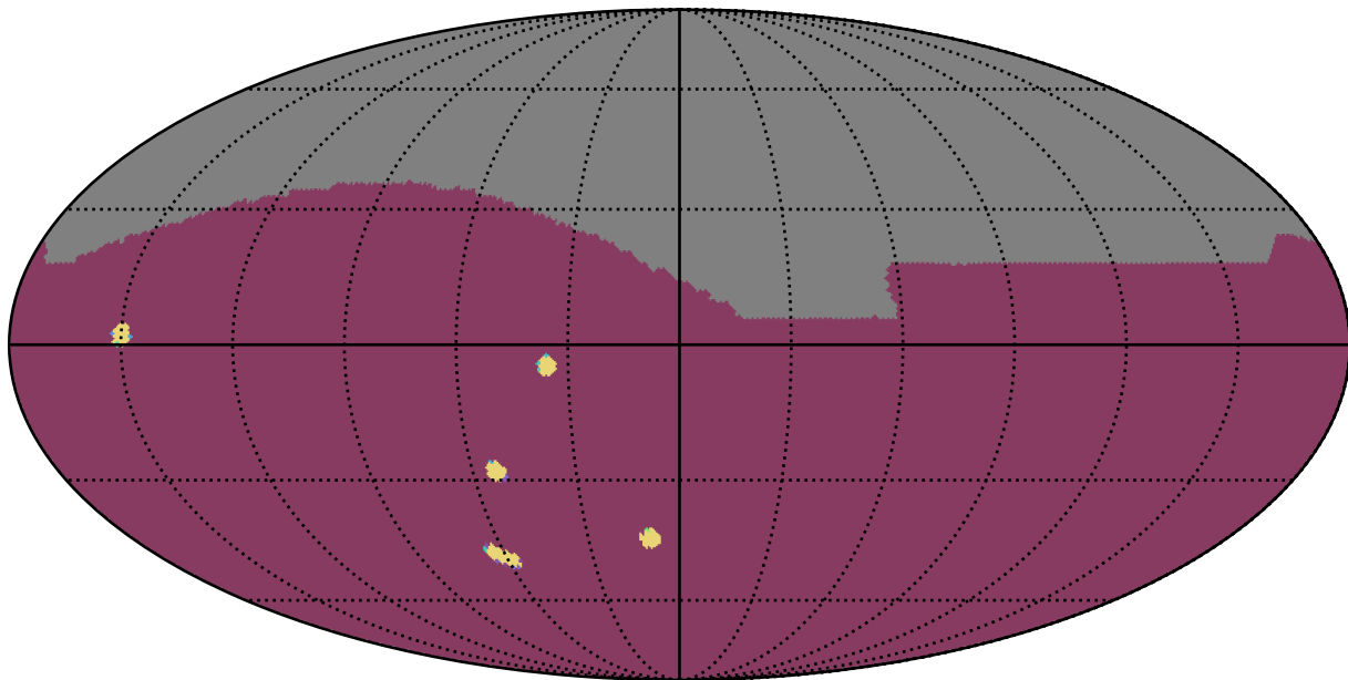
early_u_fpextra4.0_v3.4_10yrs : NumberOfQuickRevisits
