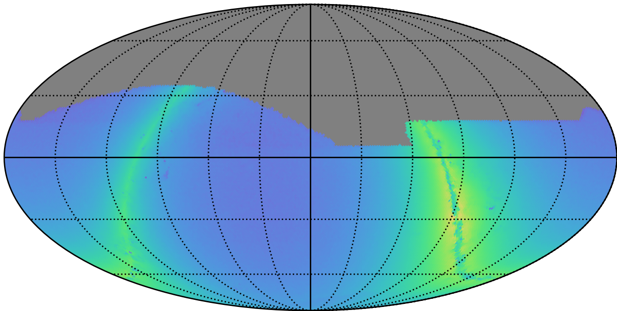
early_u_fpextra4.0_v3.4_10yrs z: Nstars_no_crowding
