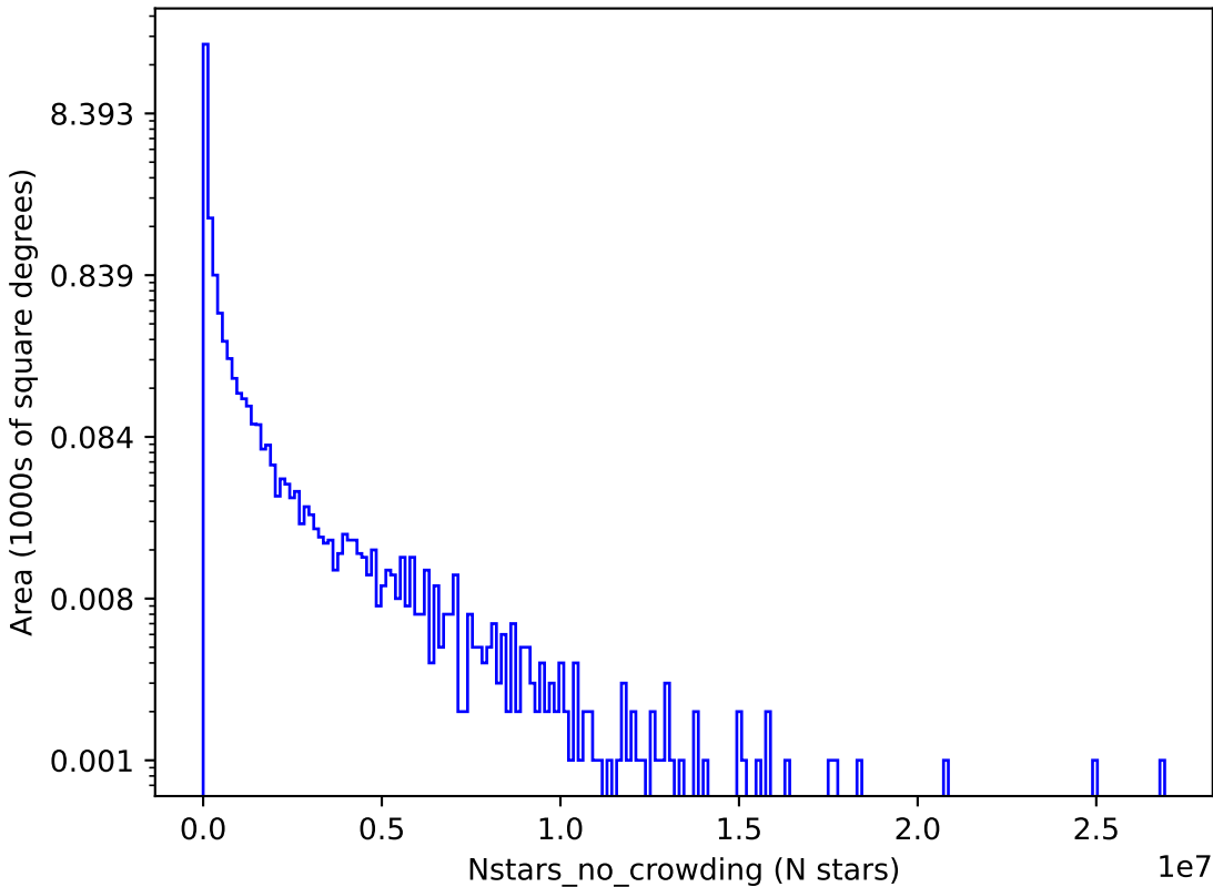
early_u_fpextra4.0_v3.4_10yrs z: Nstars_no_crowding
