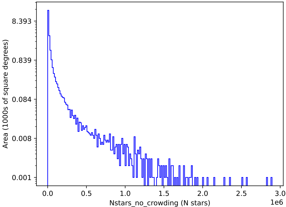
early_u_fpextra4.0_v3.4_10yrs u: Nstars_no_crowding
