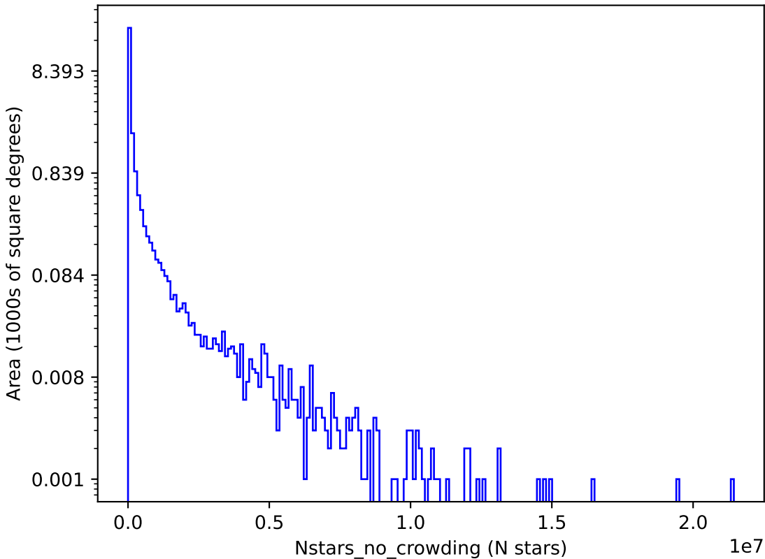
early_u_fpextra4.0_v3.4_10yrs r: Nstars_no_crowding
