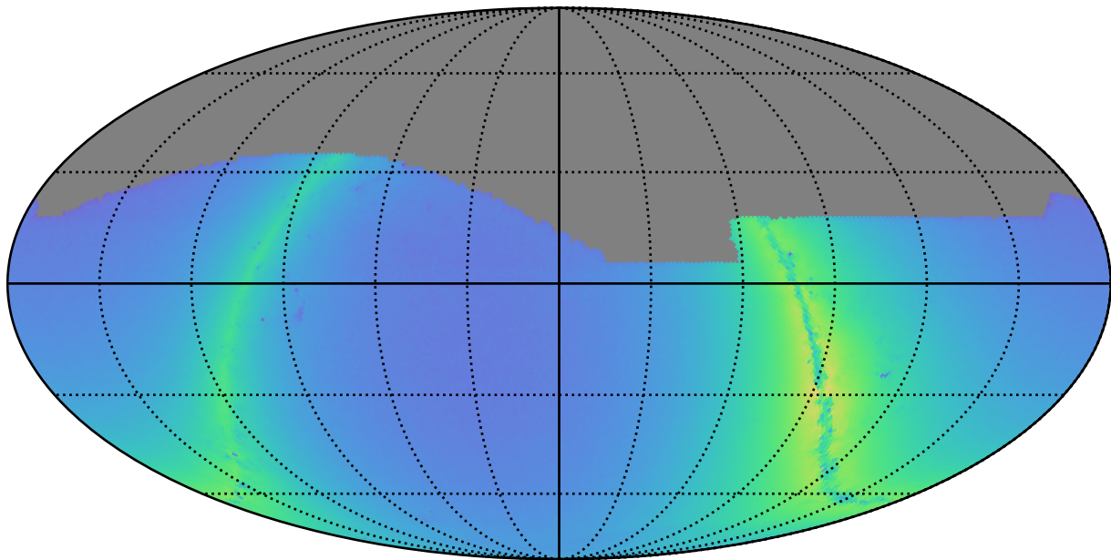
early_u_fpextra4.0_v3.4_10yrs i: Nstars_no_crowding
