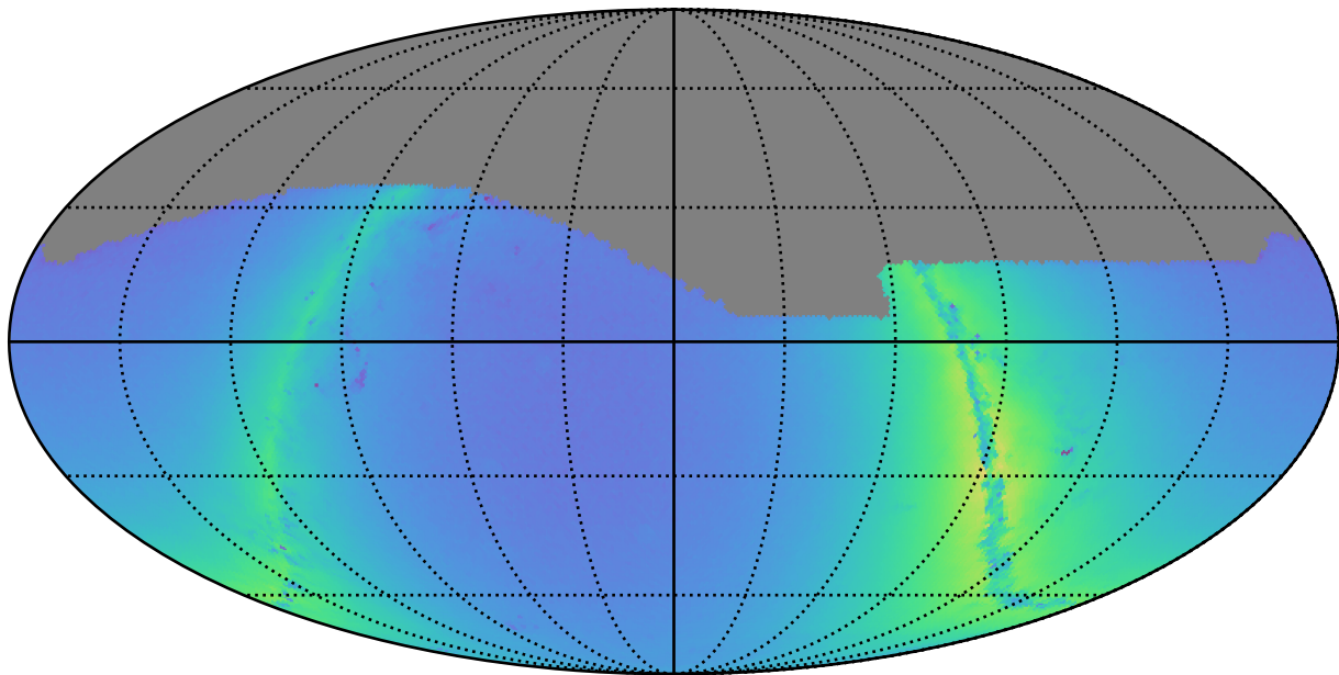
early_u_fpextra4.0_v3.4_10yrs g: Nstars_no_crowding
