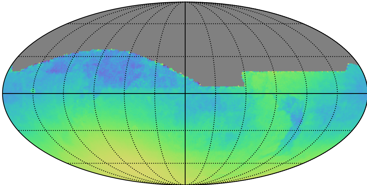
early_u_fpextra4.0_v3.4_10yrs : Normalized Parallax Uncert @ 24.0
