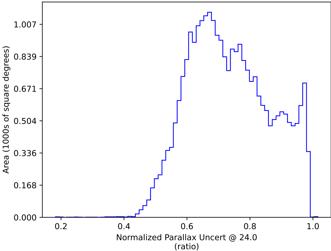
early_u_fpextra4.0_v3.4_10yrs : Normalized Parallax Uncert @ 24.0
