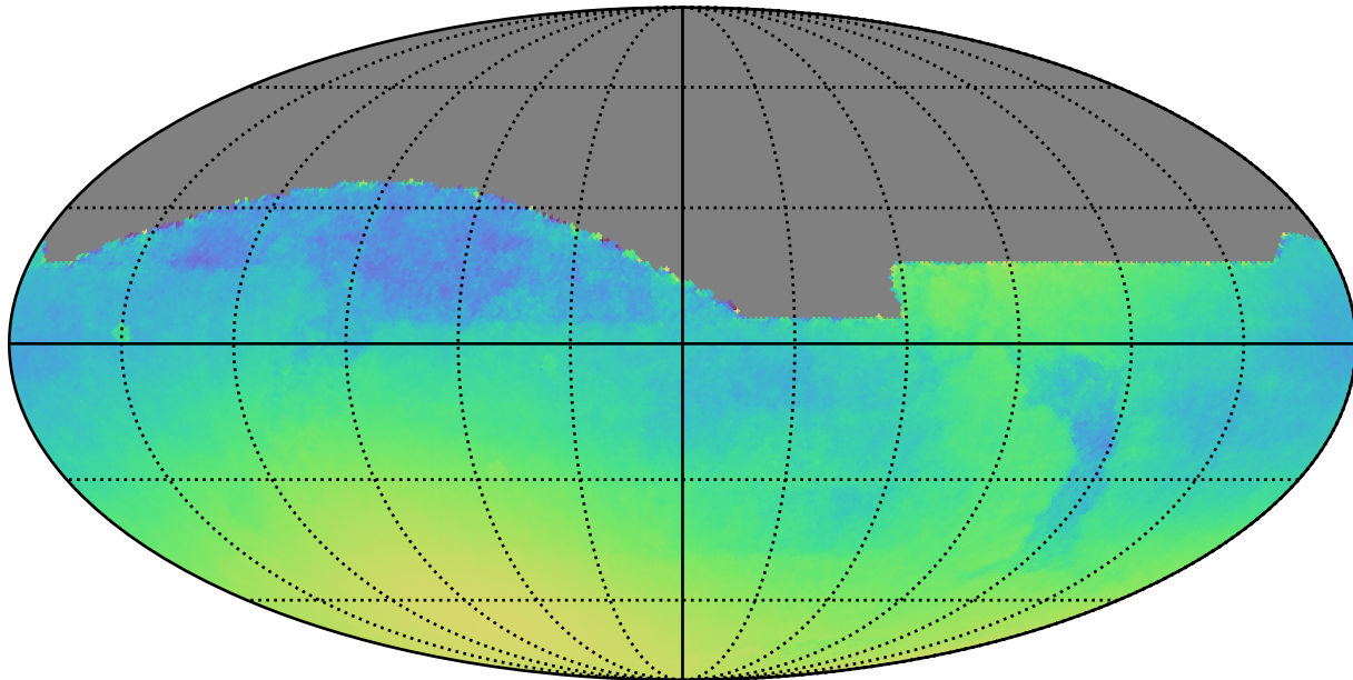
early_u_fpextra4.0_v3.4_10yrs : Normalized Parallax Uncert @ 22.4
