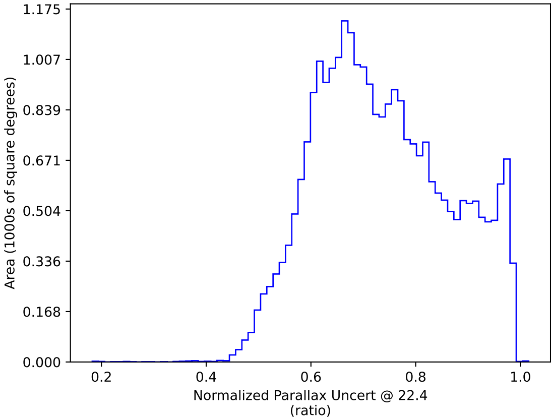
early_u_fpextra4.0_v3.4_10yrs : Normalized Parallax Uncert @ 22.4
