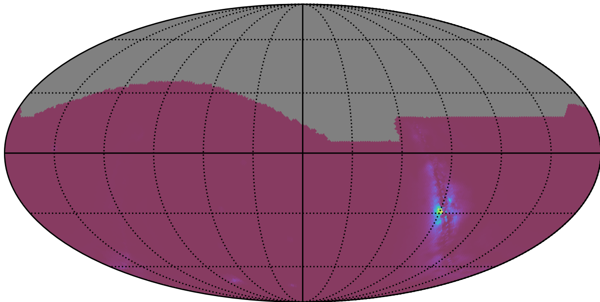
early_u_fpextra4.0_v3.4_10yrs : NlcPoints
