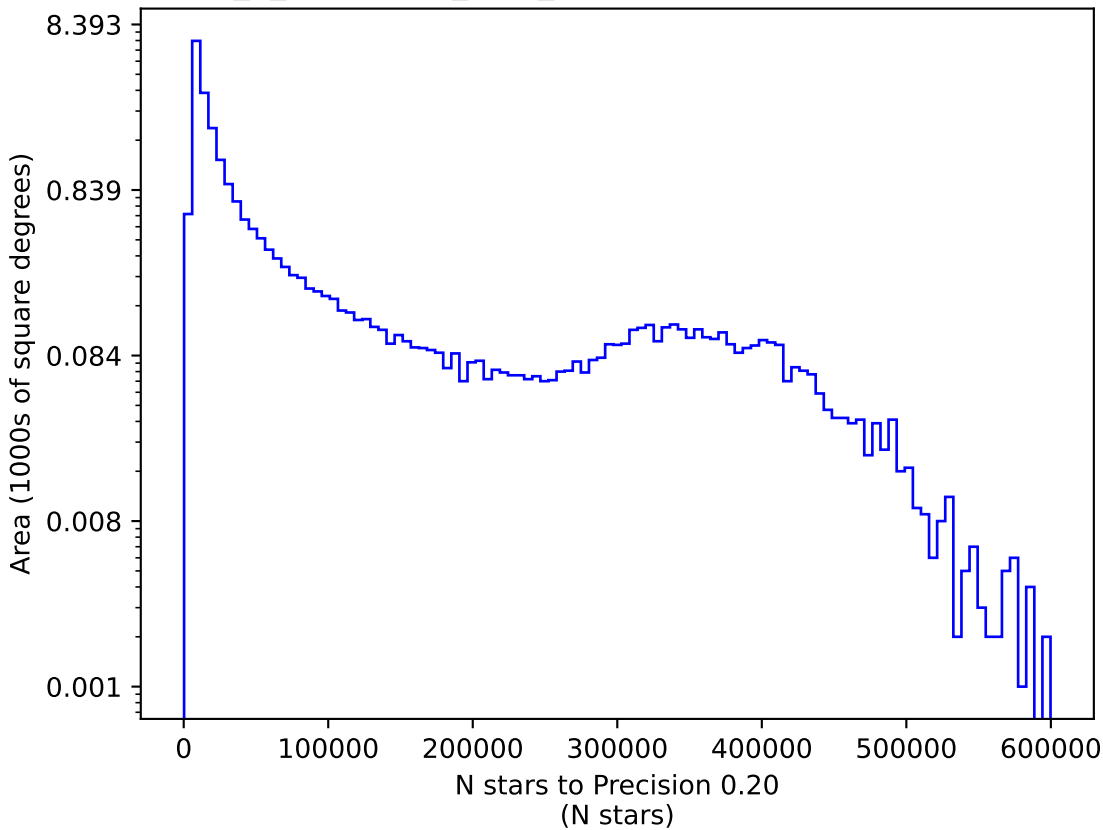
early_u_fpextra4.0_v3.4_10yrs y: N stars to Precision 0.20
