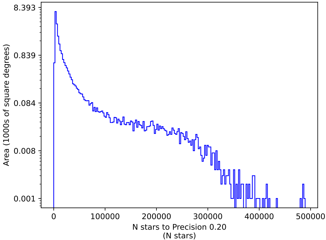
early_u_fpextra4.0_v3.4_10yrs u: N stars to Precision 0.20
