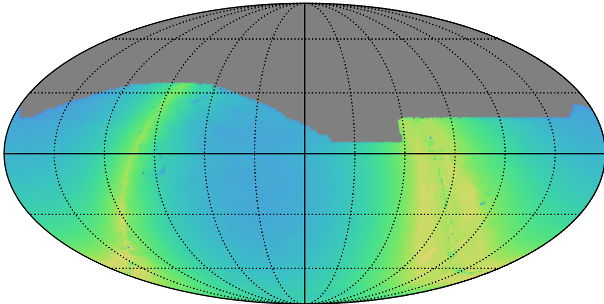
early_u_fpextra4.0_v3.4_10yrs r: N stars to Precision 0.20
