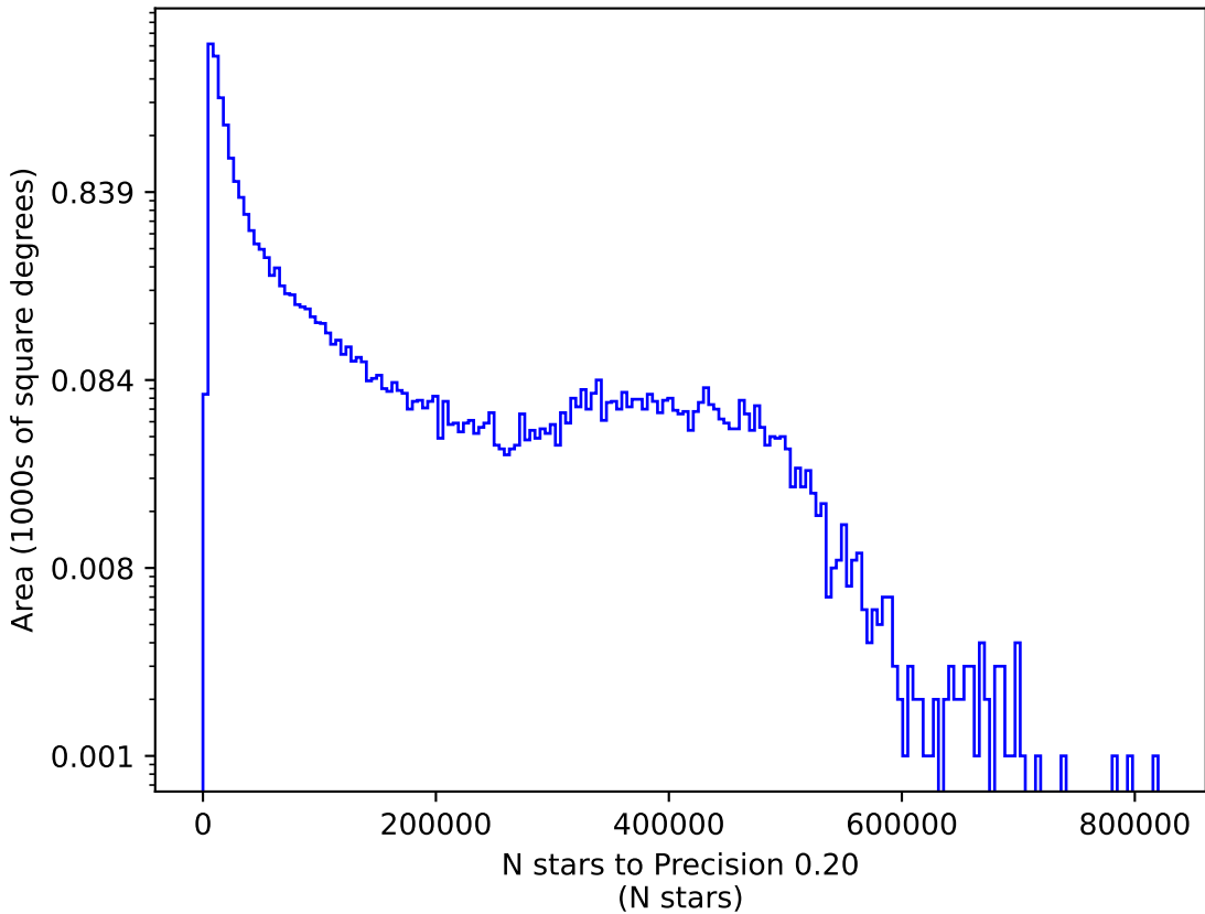
early_u_fpextra4.0_v3.4_10yrs r: N stars to Precision 0.20
