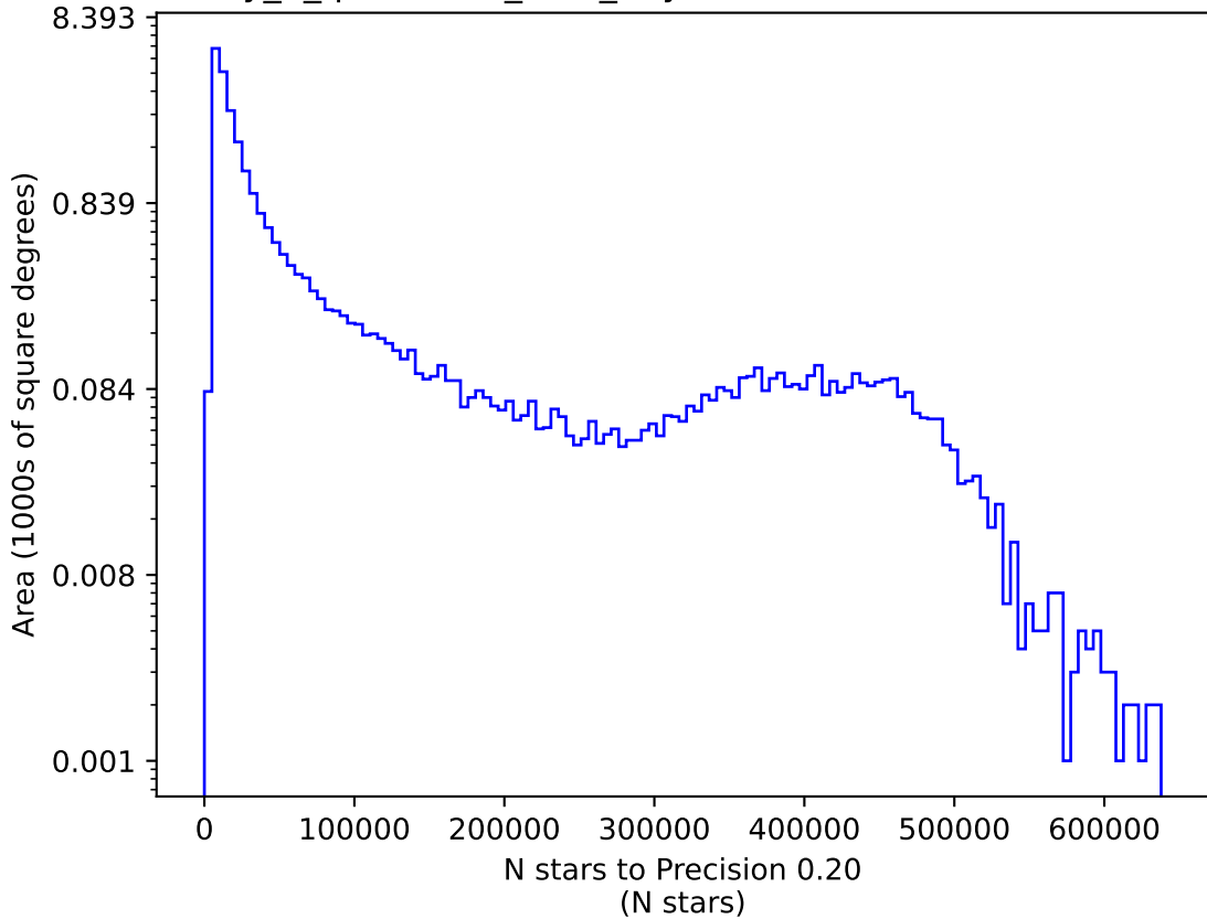
early_u_fpextra4.0_v3.4_10yrs i: N stars to Precision 0.20
