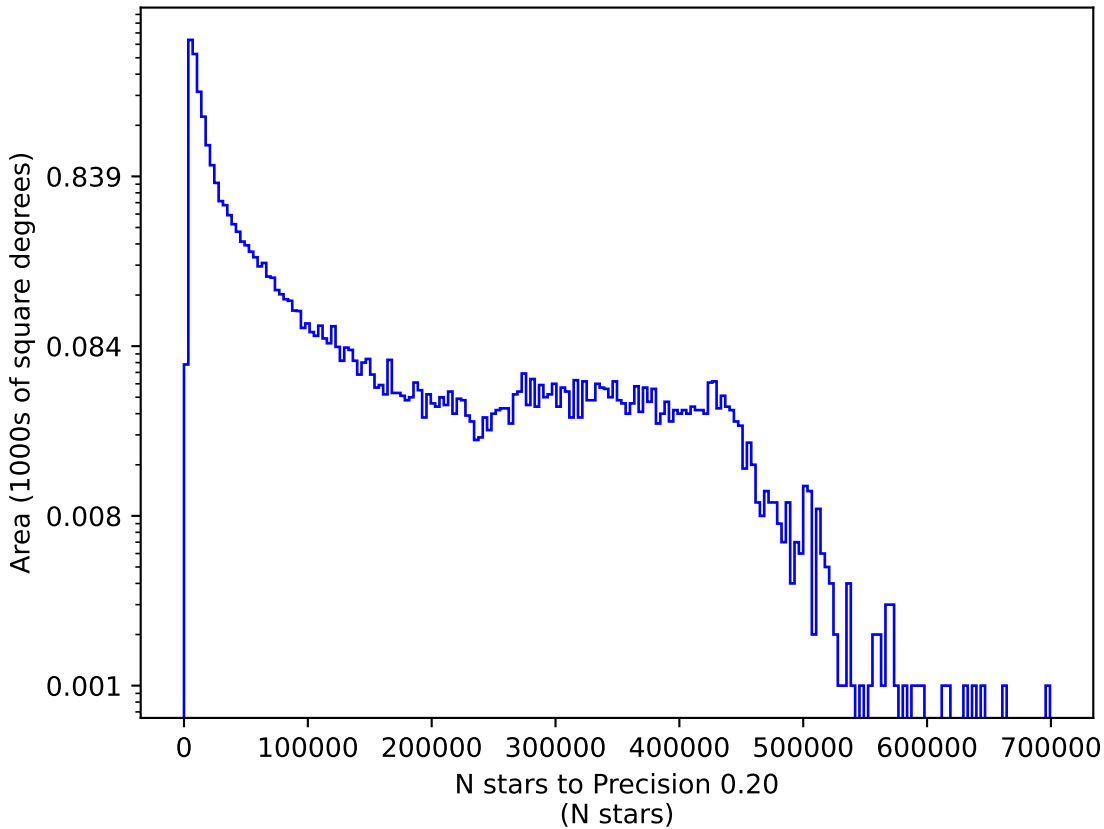
early_u_fpextra4.0_v3.4_10yrs g: N stars to Precision 0.20
