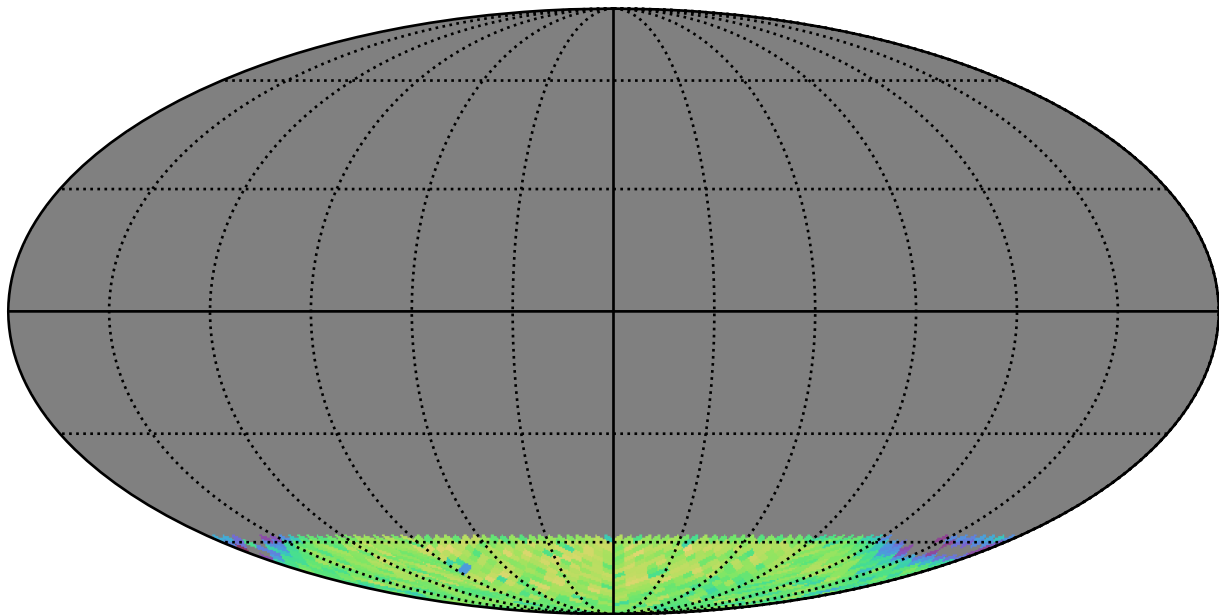
early_u_fpextra4.0_v3.4_10yrs gi SCP: LVDwarfs
