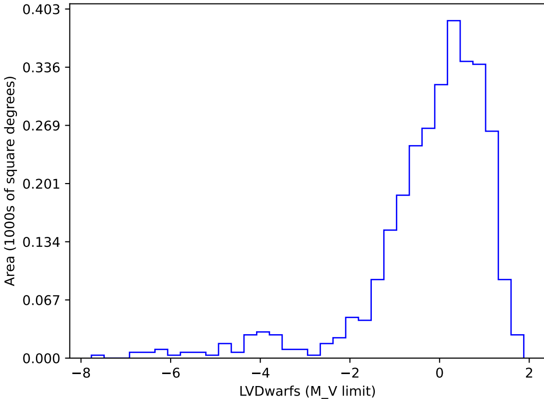
early_u_fpextra4.0_v3.4_10yrs gi SCP: LVDwarfs
